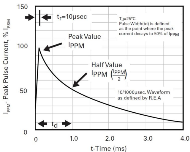
Pulse Waveform
